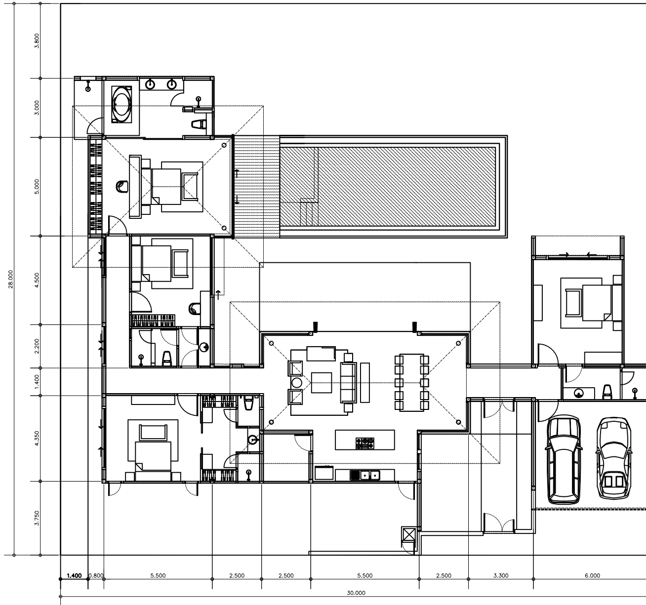
4 bedroom plan
