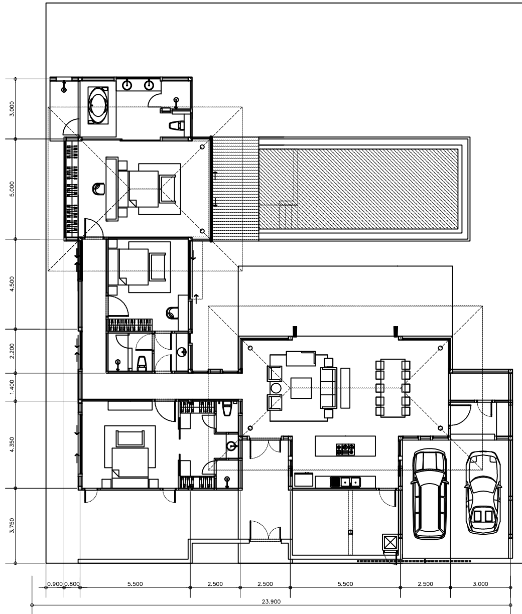
3 bedroom plan
